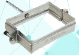
Square Downpipe Holderbat 028367 100mm X 75mm
