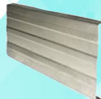
Facia Steel Chromoprep 078235 3600mm X 225 X 0.4mm 078239 4800mm X 225 X 0.4mm 078236 6000mm X 225 X 0.4mm
